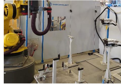
Clinching
